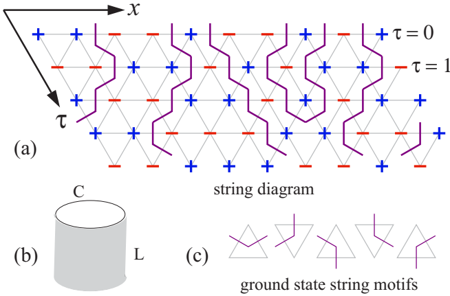
FIG. 1. (a) When each bond belongs to a unique down-pointing triangle ( \nabla ), a ground microstate has exactly one unsatisfied bond in each \nabla , but it may have three in a \Delta . Relative to the ground reference microstate, all spins up (down) on even (odd) rows, any microstate is represented up to global spin flip by the boundaries (purple “strings” here) between regions matching the reference microstate and its global spin flip. Strings cannot terminate inside the system. (b) Cylindrical geometry. (c) Motifs allowed in string representations of ground microstates. The leftmost motif corresponds to pair annihilation when strings are interpreted as particle worldlines.
