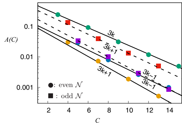
FIG. 3. Amplitudes of the asymptotic decay of end-to-end mutual information break into families labeled by \mathcal{N} parity and mod 3 residue class of C ( 3k + m , m = 0, \pm 1 ). Within each family, A(C) decays approximately exponentially in C .
