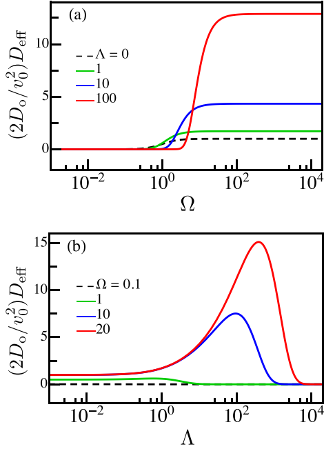
FIG. 4. Dependence of effective diffusivity on rotational \Omega and inertia \Lambda parameters.
