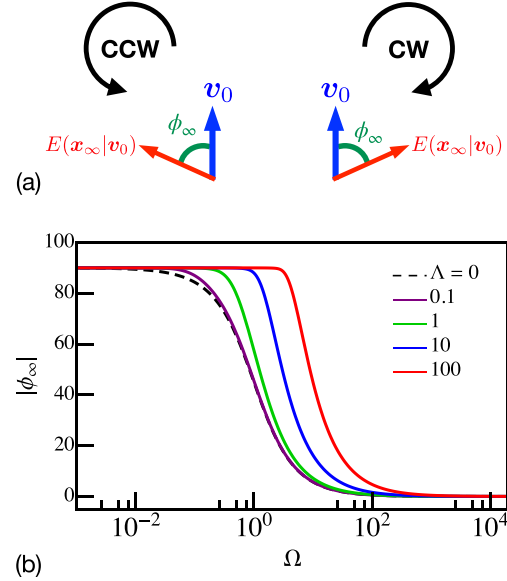
FIG. 2. (a) Dependence of expected displacement on chiral angle. (b) Absolute value of the chiral angle |\phi_\infty| as a function of D_o \tau_o for different values of correlation time.
